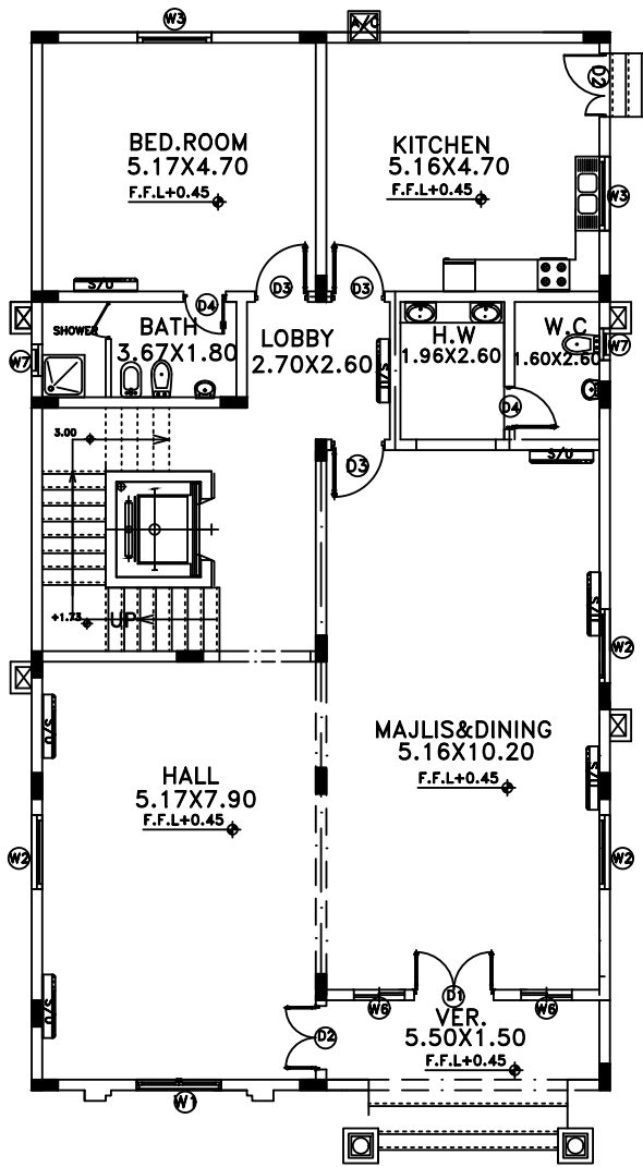
GROUND FLOOR PLAN SECALE:1/100
