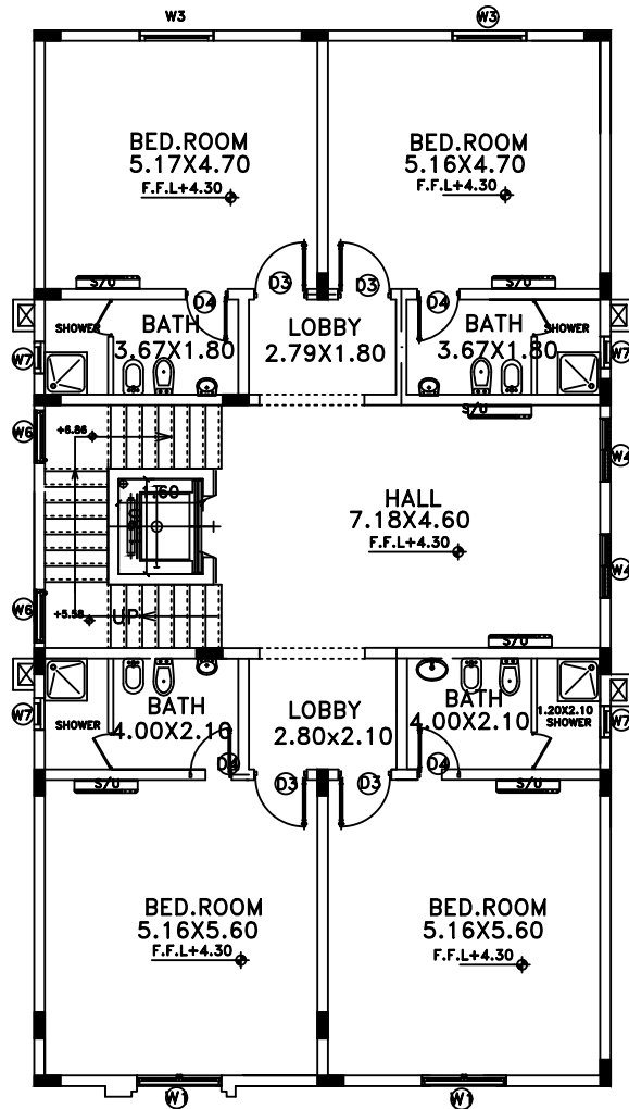
FIRST FLOOR PLAN SECALE:1/100
